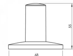
VENTIL / VALVE
