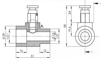
HOLENDER / ADAPTOR
