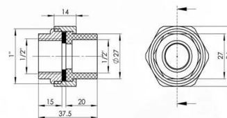
HOLENDER / ADAPTOR
