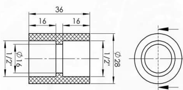
MUF / SOCKET
